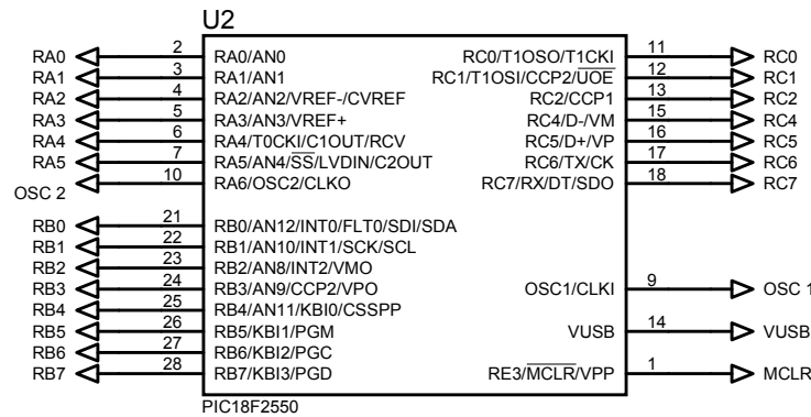
MotherBoard 2.1 Truehole
